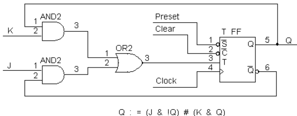
JK Flip-flop Emulation Using T Flip-flop
