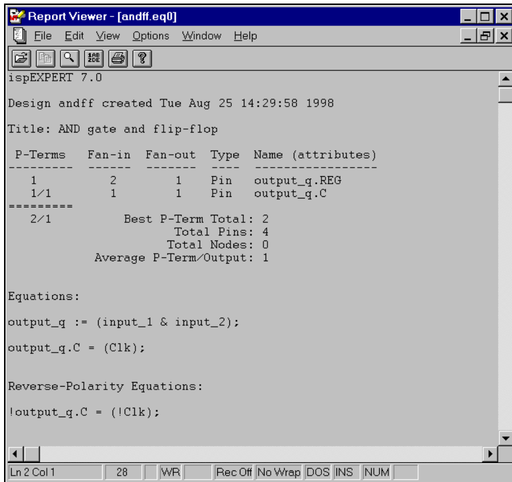
Figure 3-8. Compiled Equations for ANDFF
