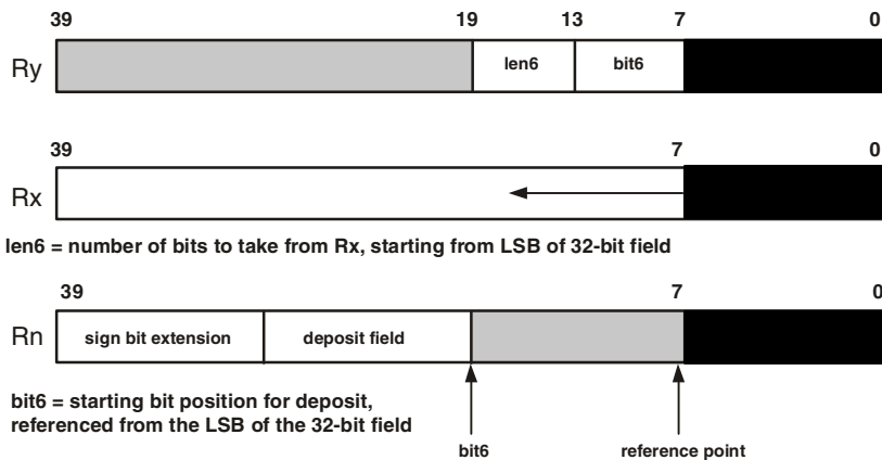
Figure 7-2. Field Alignment
